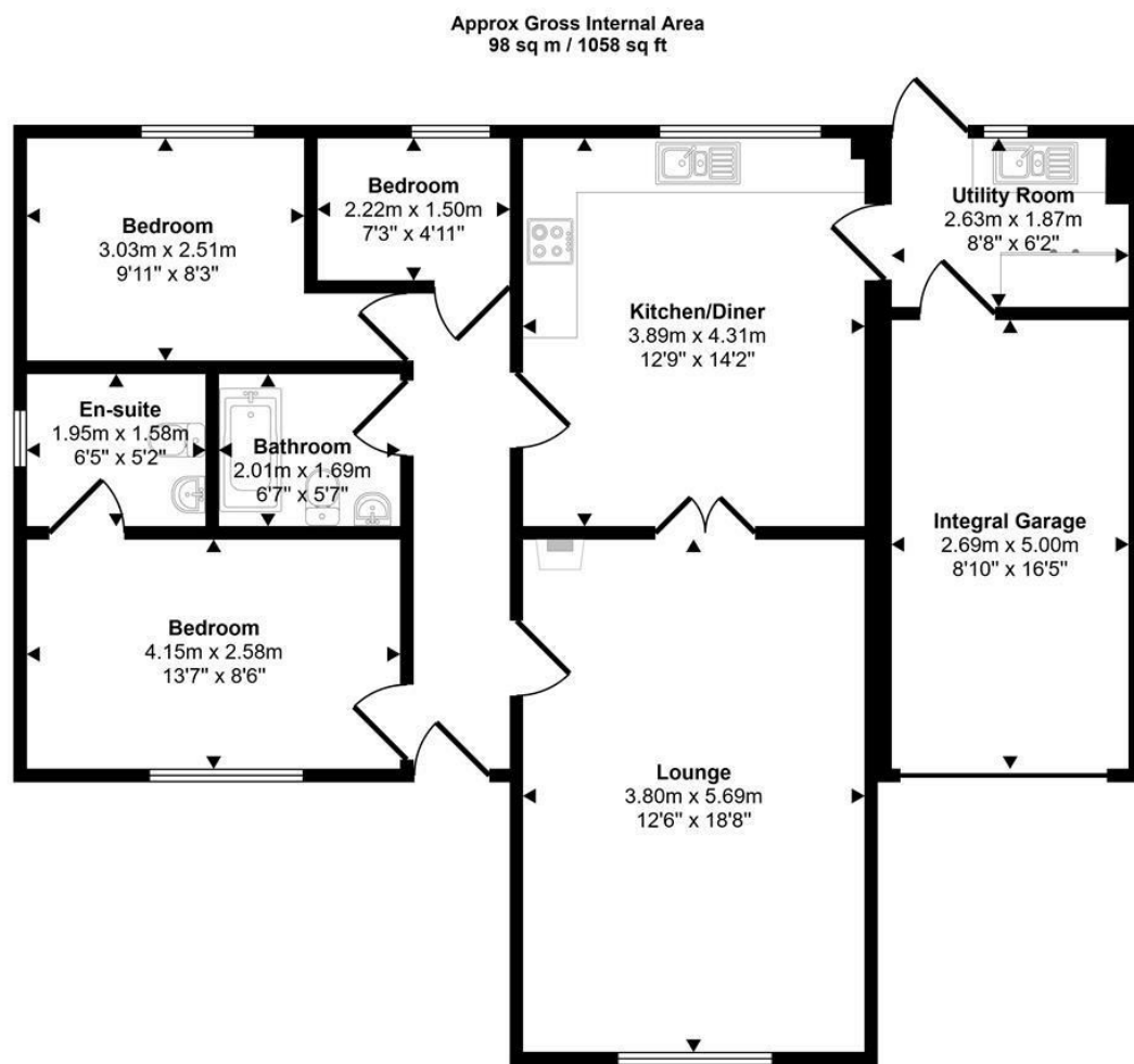
Floorplan
